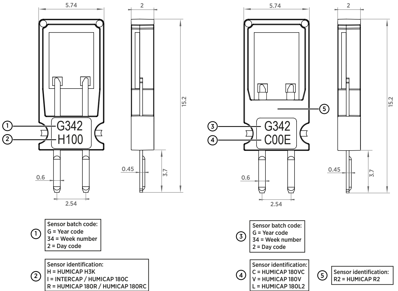
Type C (left) and type D (right) encapsulation dimensions
